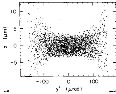
Fig. 4. Results of ray-tracing showing the correlation between the output horizontal position ( x_0 ) at the IR and input vertical angle ( y'_i ) from the collider lattice.
