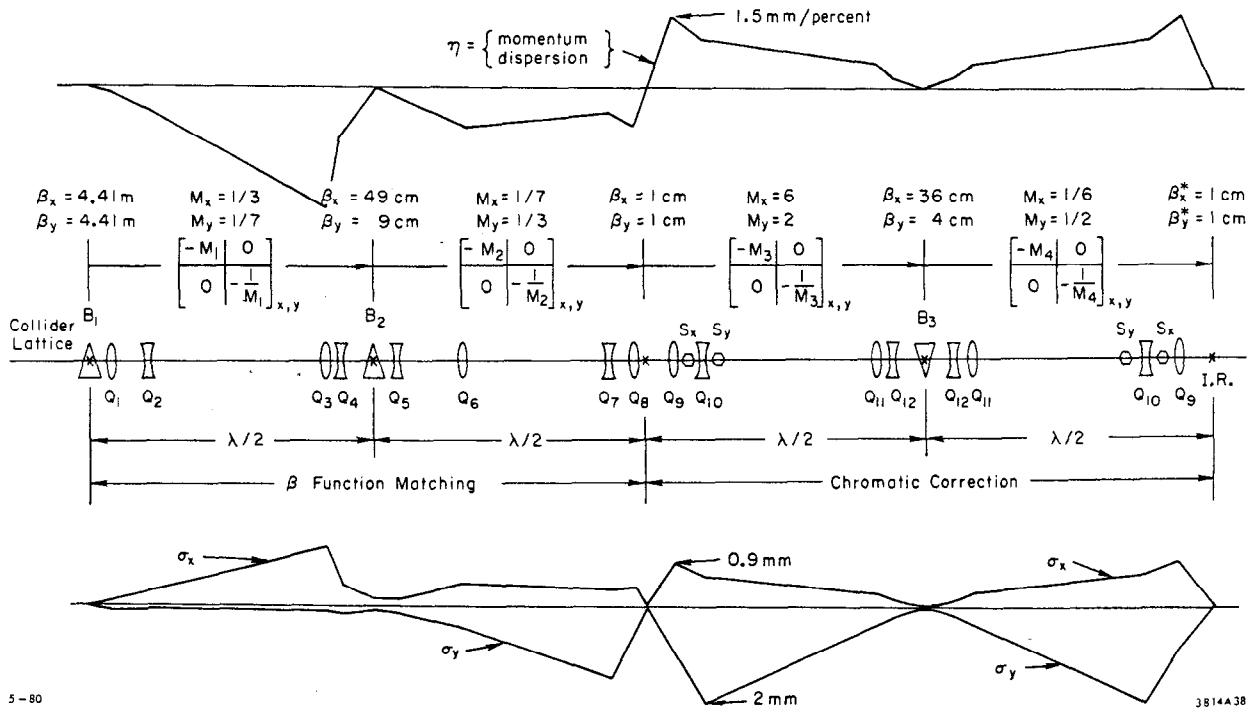
Fig. 1. Optical layout of the FFS showing the dispersion function ( \eta_x ) and betatron amplitudes ( \beta_{x,y} ).
