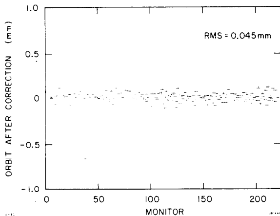
Fig. 4. Distribution of the positron beam position after correction. The distribution of the electron beam position is similar and has the same rms value as e^+ .
