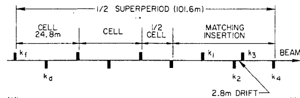
Fig. 1. Half-superperiod of the linac quadrupole lattice.
