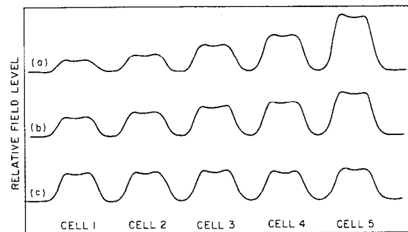
Fig. 3. Measured field profile of five cavity cells as a function of the tuners' insertion. (a) Tuner #1 inserted 10 mm, tuner #5 withdrawn 10 mm. (b) Tuner #1 inserted 5 mm, tuner #5 withdrawn 5 mm. (c) Flat field.
