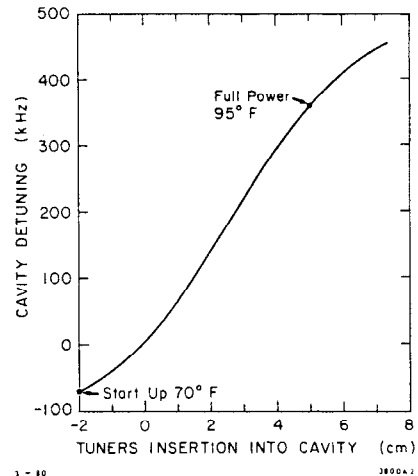
Fig. 2. Cavity tuning curve for two ganged tuners.
