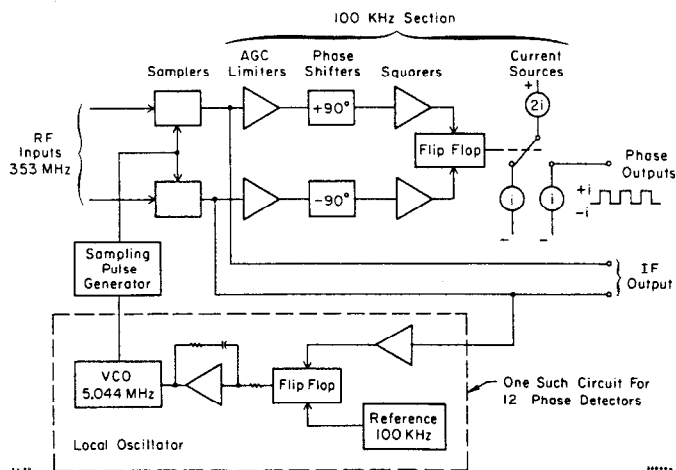
Fig. 5. Principle of the phase detectors.
