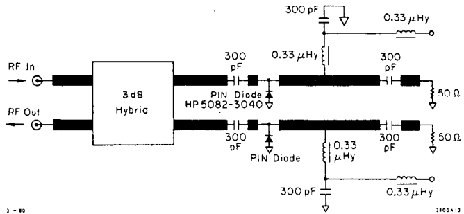
Fig. 10. Variable attenuator circuit diagram.
