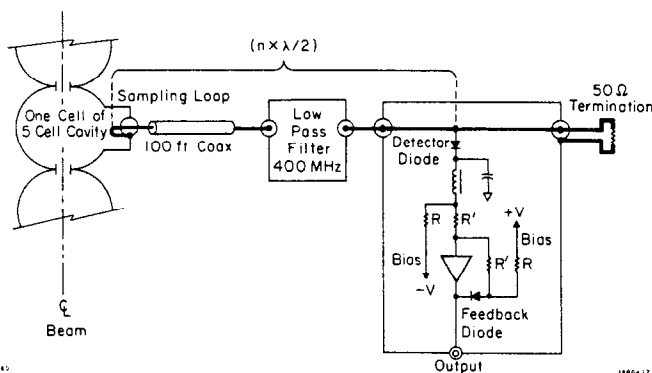
Fig. 9. RF amplitude detector circuit diagram.
