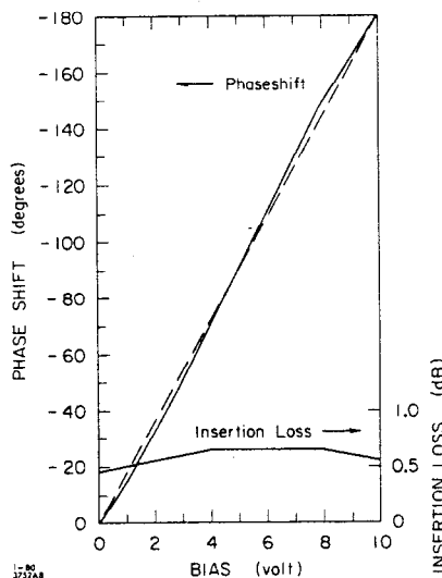
Fig. 7. Phase-shifter response and insertion loss as a function of bias voltage.
