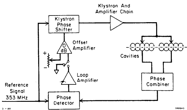
Fig. 4. Circuit of the phase control loop.
