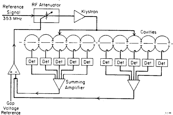
Fig. 8. Block diagram of the amplitude feedback loop.
