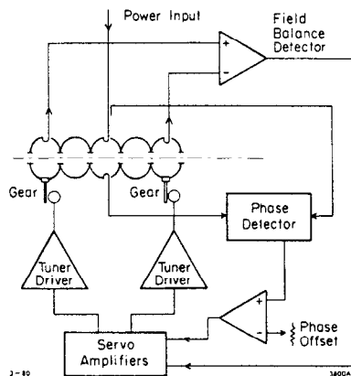
Fig. 1. Block diagram of the cavity servo loops.
