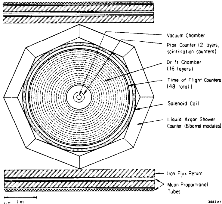
Fig. 1. Schematic view of the Mark II detector.
