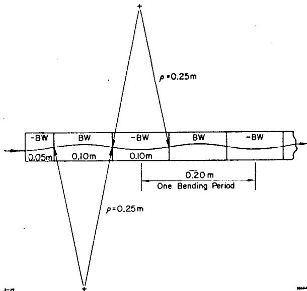
Fig. 4. Schematic of wiggler magnet.
