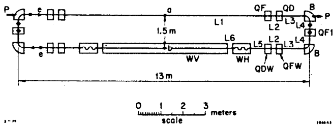
Fig. 3. Lattice of electron storage ring or cooling protons.
