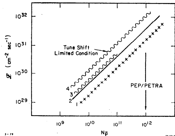
Fig. 2. Luminosity for 1000 GeV proton-antiproton storage ring as a function of N_{\bar{p}} , \Delta v and \beta^* . (1) \beta^* = 2.5 , \Delta v = 0.005 ; (2) \beta^* = 2.5 , \Delta v = 0.01 ; (3) \beta^* = 1 , \Delta v = 0.005 ; (4) \beta^* = 1 , \Delta v = 0.01 .
