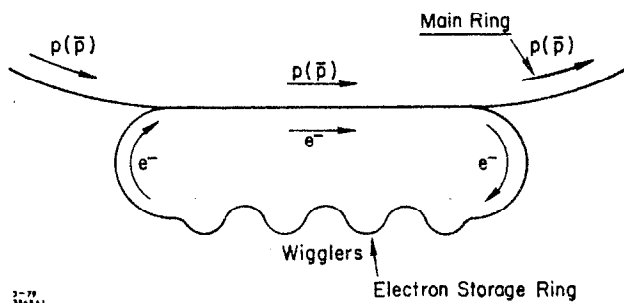
Fig. 1. High energy electron cooling plan.
