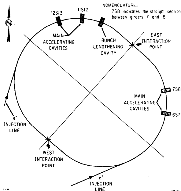
Fig. 1. Layout of RF cavities in SPEAR.
