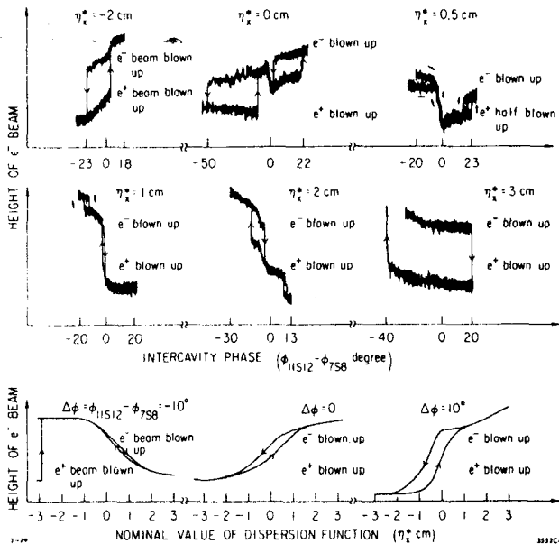
Fig. 2. Hysteresis Loops. Beam height vs intercavity phase and dispersion function.
