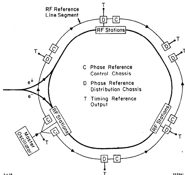
Fig. 1. PEP RF reference line layout.
