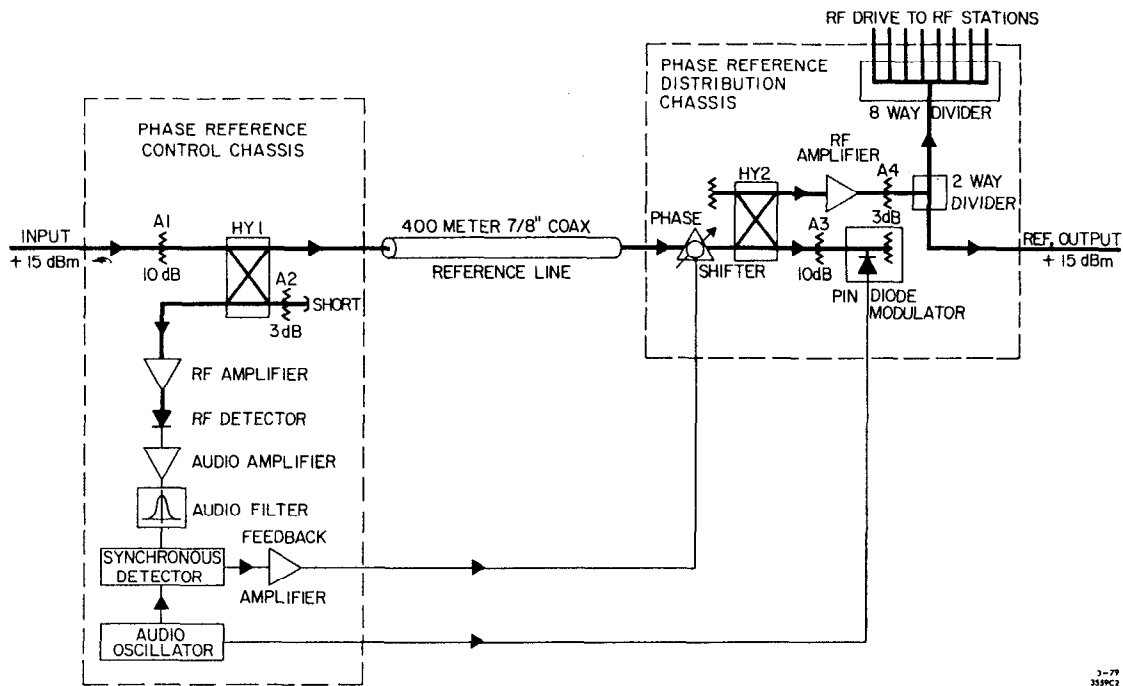
Fig. 2. RF reference line segment.
