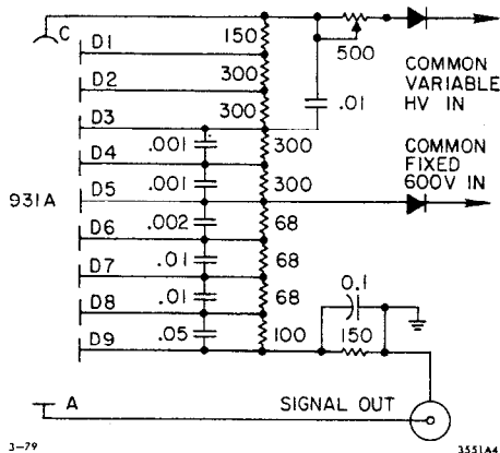
Fig. 2. Photomultiplier circuit proportioned for high peak current output. Values are in \mu\text{F} and \text{k}\Omega .
