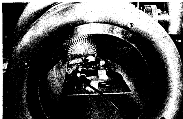
Fig. 3 shows the gun, pulser, and power supply electronics in place in a test facility, and Fig. 4 shows the pulser board in the gun cone.
