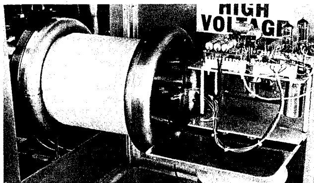
Fig. 3 shows the gun, pulser, and power supply electronics in place in a test facility, and Fig. 4 shows the pulser board in the gun cone.
