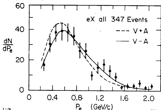
Fig. 4. Electron momentum spectrum from eX events, all energies. The curves are detailed Monte Carlo generated fits.
