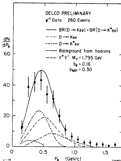
Fig. 7 Electron momentum distribution for multiprong electron events at the \psi'' .
