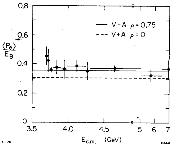
Fig. 5. Average scaled electron momentum
