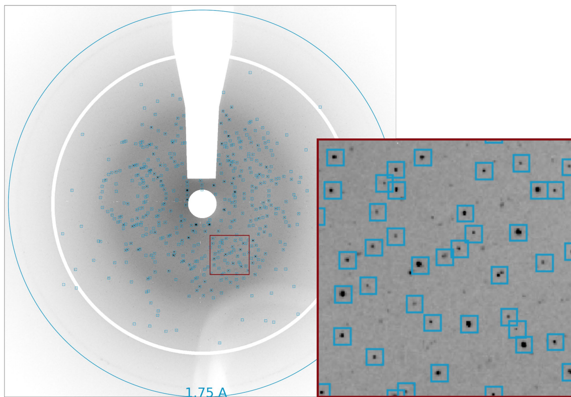
Figure 2 A diffraction pattern from a single drop containing multiple Thaumatin crystals (Run 31). Blank areas represent masked out pixels where shadow from the nozzle and diffraction from copper shielding are removed prior to peak finding. Dark spots represent Bragg peaks, and blue squares indicate peaks found by Psocake .
