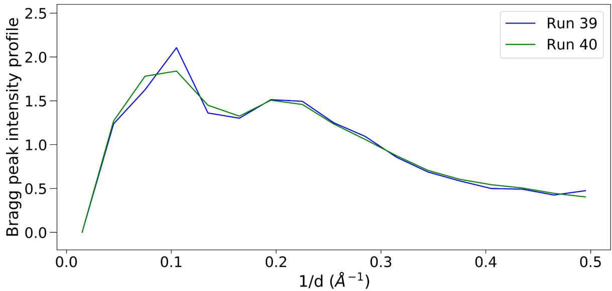
Figure 8 Radially averaged Bragg peak intensity profiles up to \sim 2\text{\AA} for run 39 and 40. The per-image radial profile of a single pattern was calculated by averaging Bragg peaks identified by Psocake in each shell, which was further scaled to minimize the L_2 distance to the reference radial profile of the first hit in the same run. The radial profile curve of a whole run, as shown in this plot, was calculated by averaging these scaled per-image radial profiles of all hits in this run. For improved comparison, both curves of run 39 and 40 are scaled to have a mean value of 1.
