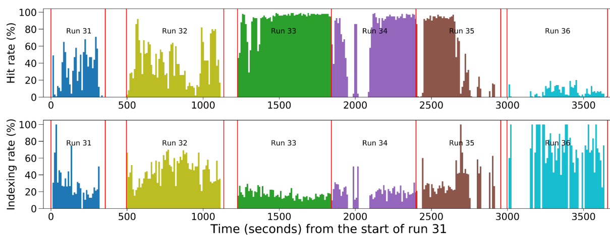
Figure 6 The continuous hit and indexing rates from the start of run 31 to the end of run 36. The data are colored based on run numbers and divided by red vertical lines indicating the start and end time points of each run. Neighboring runs being divided by two red vertical lines indicates an interval between these two runs, for example, there is a 139-second time interval for wash between run 31 and 32. Each small time bin is 10-second long. The hit rate is defined as the percentage of hits identified by Psocake among all diffraction patterns collected in each time bin, and the indexing rate here is the ratio of indexed events to the number of hits in each time bin, with multiple-crystal hits counted once.
