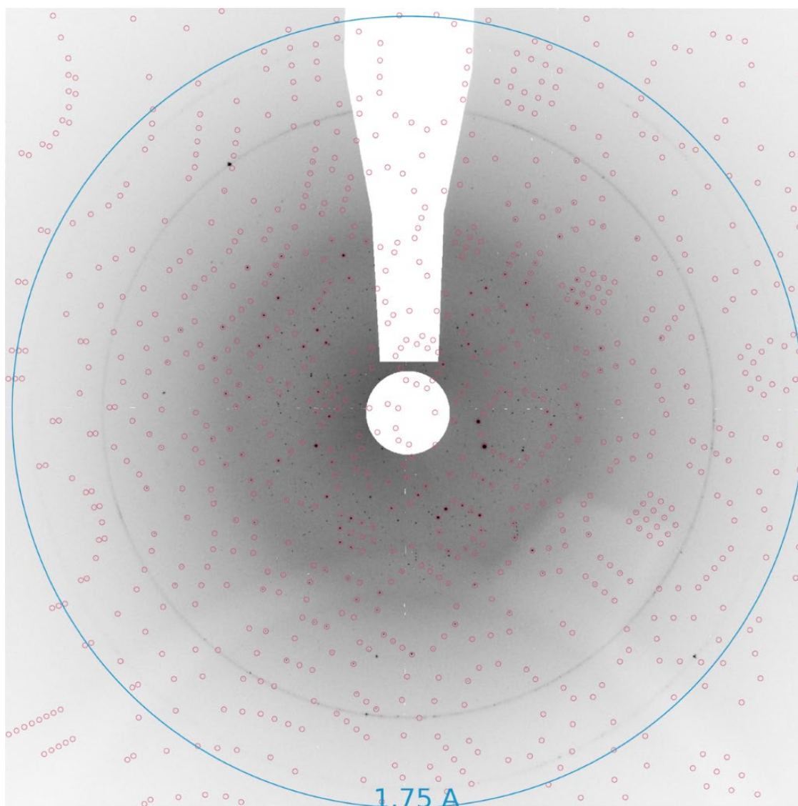
Figure 3 A diffraction pattern from Thaumatin and predicted spots from indexing (Run 31). Black dots are possible Bragg peaks, and red circles indicate predicted Bragg peak positions indexed by indexamajig in CrystFEL (White et al. , 2012, 2016).
