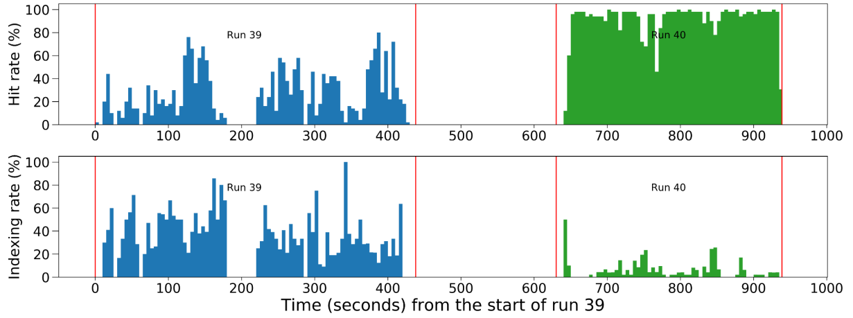
Figure 7 The continuous hit and indexing rates from the start of run 39 to the end of run 40. The data are colored based on run numbers, with the start and end time points of each run labelled with red vertical lines. Each small time bin is 5-second long, and there is a 192-second time interval between these two runs. The hit and indexing rates are calculated using the same method as described in Fig. 6.
