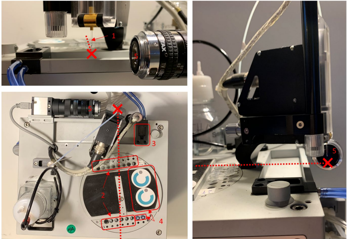
Figure 1 Setup of the dispense system. (1) represents the nozzle just above the interaction point (marked with red cross), (2) indicates the sample and buffer tube holders, (3) is the tip wiping station, (4) is the nozzle washing station, and (5) is the drop camera. The beam path is represented with the red dashed line and interaction point with the red cross.
