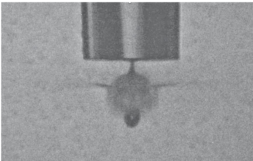
Figure 5 The tail of the droplet shown exploding as it is intercepted by an FEL pulse.
