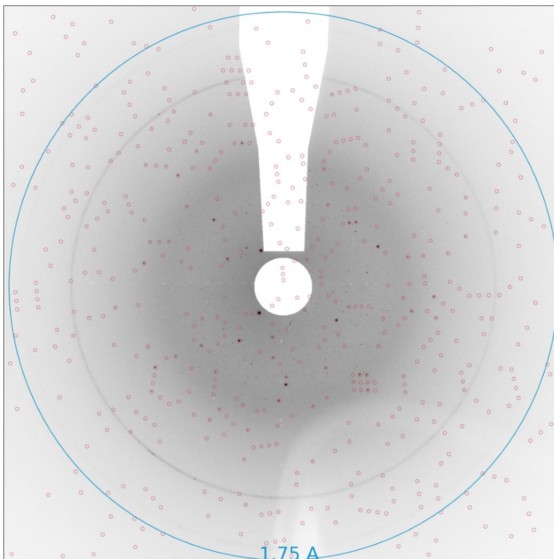
Figure 4 A diffraction pattern from Thaumatin and predicted spots from indexing (Run 39). Black dots are possible Bragg peaks, and red circles indicate predicted Bragg peak positions.
