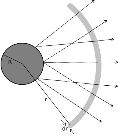
FIG. 1. Schematic picture of neutrino emission from the proto-neutron star, and the neutrino ensemble represented by the density operator \hat{\rho}_t(E, r)dt dE in the neutrino bulb model [23]. See the text for details.
