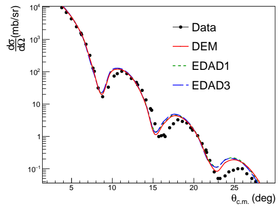
FIG. 6. Differential cross section for elastic proton scattering on ^{40}\text{Ar} at 0.8 GeV as a function of scattering angle. Results for the DEM, EDAD1, and EDAD3 optical potentials, which turn out to almost completely overlap, are compared with the experimental data [72].
