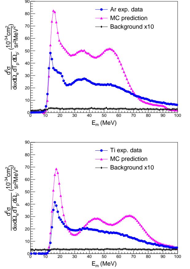
FIG. 3. Six-fold differential cross section as a function of missing energy for argon (top panel) and titanium (bottom panel). The background estimate (line connecting the experimental data points) is multiplied by 10 for purpose of presentation. The MC predictions, based on the mean-field SF, include a correction for the nuclear transparency, while other FSI effects are not accounted for.
