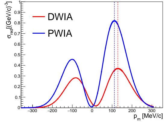
FIG. 5. Reduced cross section as a function of missing momentum for the 1p_{1/2} proton knockout from argon. We compare the PWIA and DWIA results obtained for the parallel kinematics considered in this analysis.
