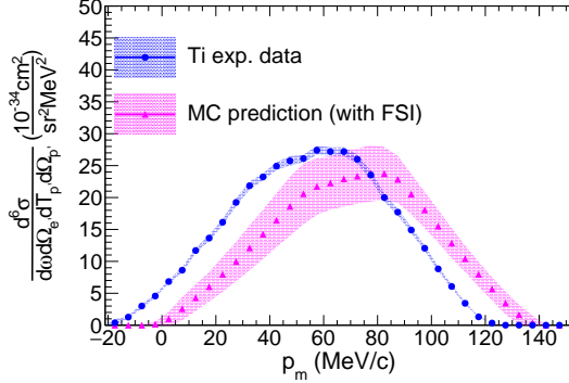
(c) 54 < E_m < 90 MeV
