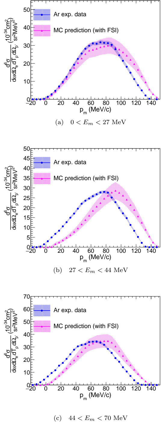
FIG. 7. Six-fold differential cross section for argon as a function of missing momentum integrated over different ranges of missing energy. The background estimate is multiplied by 10 for presentation. The MC predictions, based on the mean-field SF, include the full FSI corrections.
