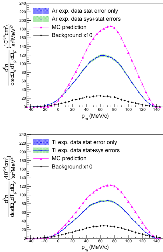
FIG. 4. Same as Fig. 3 but for the cross section as a function of missing momentum. The inner (outer) uncertainty bands correspond to statistical (total) uncertainties.
