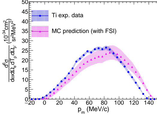
(a) 0 < E_m < 30 MeV
