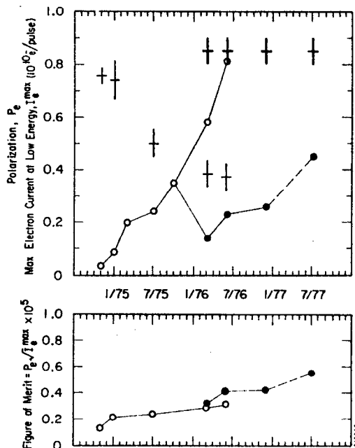
Fig. 1. PEGGY's development as a function of time and projection for the near future. The open circles and thin crosses in the upper plot are, respectively, maximum current and polarization measurements with resonant depolarization effects present. The filled dots and heavy crosses are measurements with resonant depolarization effects removed.
