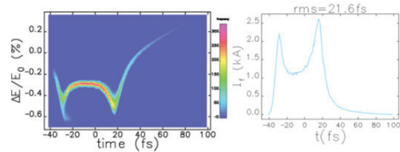
Figure 10: Phase space before undulator from Elegant simulation for 100pC beam with 1.5kA peak current.
