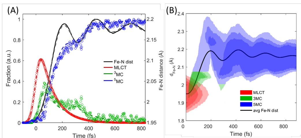
Figure 7. Simulating the experimentally determined excited state dynamics. Using the potential energy surfaces in Fig. 6(C) and the modelling described in the text, an accurate fit (dashed lines) of the excited state population dynamics extracted from the XES measurement (circles) and Fe-N ensemble
