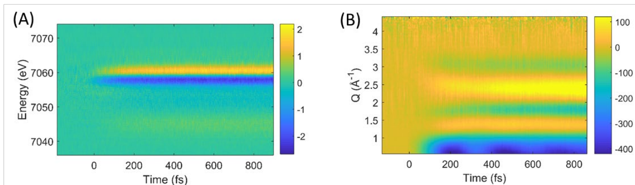
Figure 2. The time-resolved difference XES (A) and XDS (B) signals generated by photoexcitation of [Fe(bpy) 3 ] 2+ at 400 nm.
