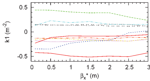
Figure 5: Strengths of the upstream IR quadrupoles vs. \beta^* .
