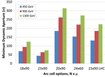
Figure 3: DA of the HE-LHC and LHC designs with \Delta p/p , without magnet errors.
