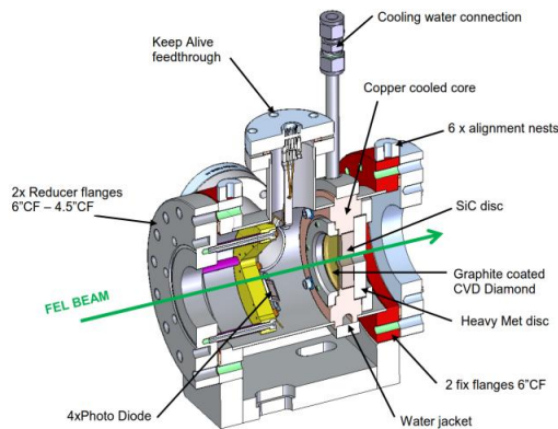
Figure 1: Photon collimator assembly section view.
