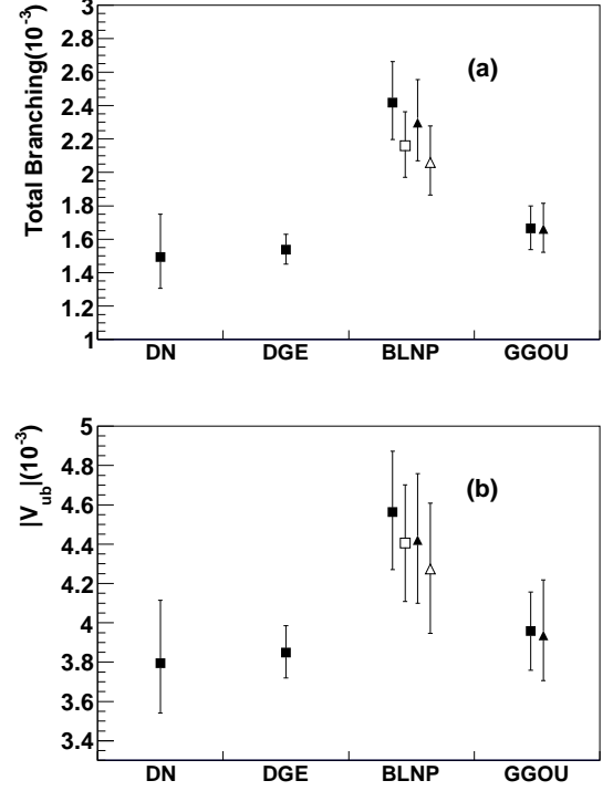
FIG. 18: Results for (a) \mathcal{B}(B \rightarrow X_u e \nu) , and (b) |V_{ub}| based on the momentum range p_e = 0.8 - 2.7 GeV/c for different QCD calculations and SF parameterizations (Table VI). For BLNP and GGOU: solid squares - X_c \ell \nu moment fits with m_c constraint (BLNP 1 and GGOU 1 ), solid triangles - X_c \ell \nu and X_s \gamma moment fits (BLNP 3 and GGOU 2 ), open squares or triangles - the same constraints for translation of SF parameters from “kinetic” to “shape-function” scheme with \mu_i = 1.5 GeV (BLNP 2 and BLNP 4 ).
