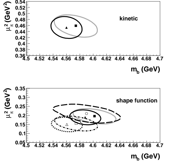
FIG. 3: The shape function parameters m_b and \mu_\pi^2 in the kinetic scheme (HFAG 2014): fit to X_c data with constraint on the c -quark mass (solid line, solid triangle); fit to X_c + X_s \gamma data ( \mu_i = 1.5 \text{ GeV} , \mu = \mu_i ) (dotted line, solid square). Translation of fit to X_c data with constraint on the c -quark mass (short dashed line, open triangle); translation of fit to X_c + X_s \gamma data with \mu_i = 2.0 \text{ GeV} , \mu = \mu_i (dash-dotted line, open square). The previous BABAR endpoint analysis [8] was based on a X_s + X_c fit (long dashed line, open circle). The contours represent \Delta\chi^2 = 1 .
