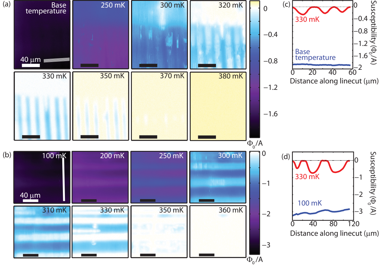
FIG. 3. Color. The spatial variation in susceptibility near T_c is much weaker at lower temperatures. (a) Repeated scans at a single location. (b) Repeated scans at a second location. White lines in (a) and (b) indicate the positions of linecuts displayed in (c) and (d), respectively. (c,d) Averaged linecuts taken at 330 mK and at base temperature (c) or at 330 mK and 100 mK (d) demonstrate that the relative amplitude of modulation of the superconducting response is larger at temperatures near T_c than at the lowest temperatures.
