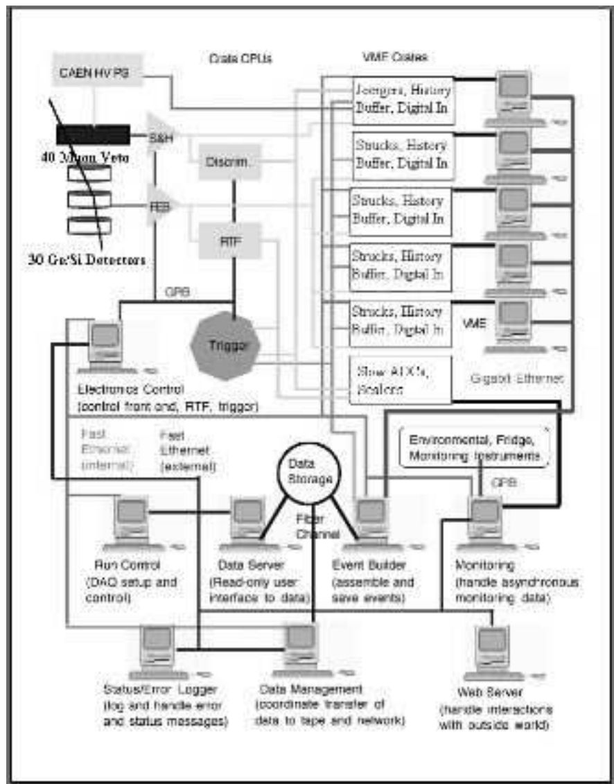
FIG. 6: CDMS-II data acquisition layout showing the various hardware components in relation to the detector and veto systems. When a detector triggers, various detector and veto elements are read out to form an event. Monitoring processes run continuously to monitor the health of the detector, veto, and cryogenics components.
