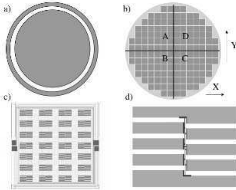
FIG. 4: Diagram of a CDMS ZIP detector. a) The “ionization side” of the detector with a large inner electrode and an outer guard ring electrode. b) The “phonon side,” divided into four quadrants labeled A, B, C, and D, each consisting of 37 dies of 28 QETs. The convention for the x-y axes is shown. The area outside the cells consists of a passive Al/W grid that is patterned sparsely (10% area coverage) to minimize athermal-phonon absorption while maintaining field uniformity for the ionization measurement. c) One of the 37 dies constituting a single phonon channel; each die contains 28 QETs. d) One of the QETs consisting of a 1- \mu\text{m} -wide tungsten strip connected to 8 aluminum fins.
