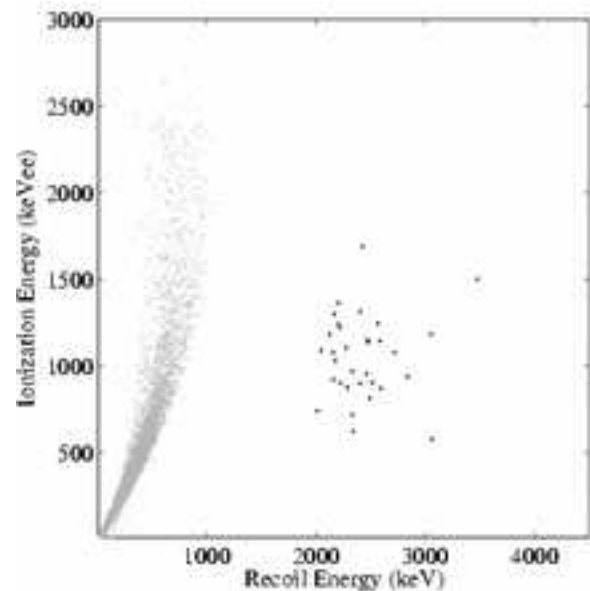
FIG. 11: Plot of ionization energy versus recoil energy for events during the WIMP search after the initiation of an old-air purge between the outer copper can and the surrounding mu-metal shield. Alphas (black dots) interacting in the detectors are easily identified. Nonlinearity in the phonon energy response at high energies is evident in the gammas (gray dots). This nonlinearity results in the recoil energy of the alphas being underestimated by about a factor of two.
