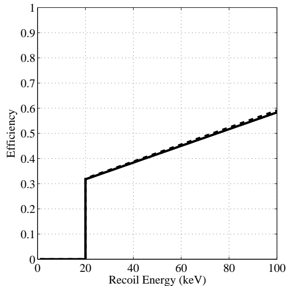
FIG. 34: Overall WIMP efficiency for the Si detector Z4. Dashed line corresponds to the efficiency for the initial analysis and the solid line is the efficiency for the current analysis. The two estimates differ by less than 1% since, for this detector, there was little difference between using the time-based pulse height algorithm and the optimal filter algorithm.
