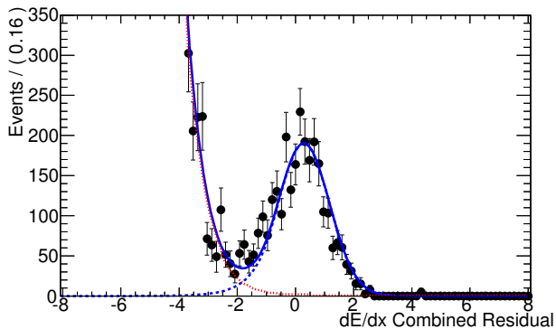
FIG. 1. Normalized residuals of the combined dE/dx for antideuteron candidates in the Onpeak \Upsilon(2S) data sample, with fit p.d.f.'s superimposed. Entries have been weighted, as detailed in the text. The solid (blue) line is the total fit, the dashed (blue) line is the \bar{d} signal peak, and the dotted (red) line is the background.
