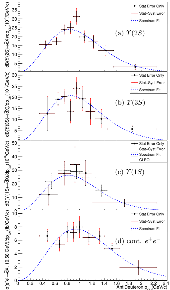
FIG. 2. Measured antideuteron differential spectra in (a) \Upsilon(2S) , (b) \Upsilon(3S) , (c) \Upsilon(1S) decays, and (d) e^+e^- \rightarrow q\bar{q} at a CM energy of \approx 10.58 GeV. The points with inner (black) error bars give the measurements and their associated statistical uncertainties, the outer (red) error bars give the quadratic sum of the statistical and systematic uncertainties, and the dashed (blue) curves show the fit to Eq. 2. Subfig. (c) also includes the CLEO results with dashed error bars for comparison.
