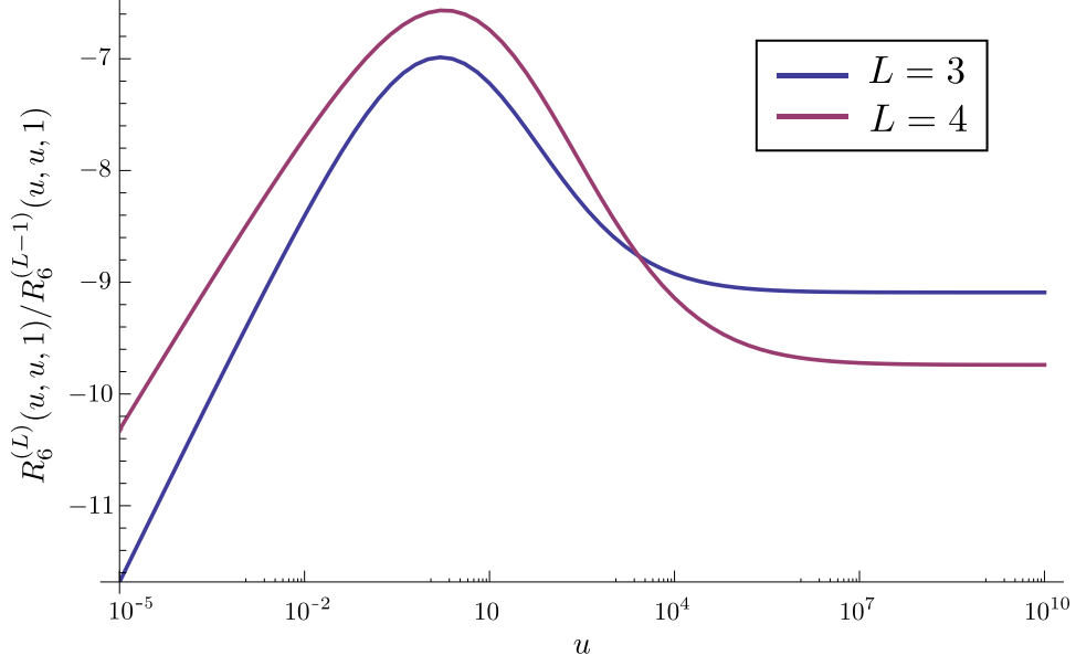
Figure 2: The successive ratios R_6^{(L)}/R_6^{(L-1)} on the line (u, u, 1) .
