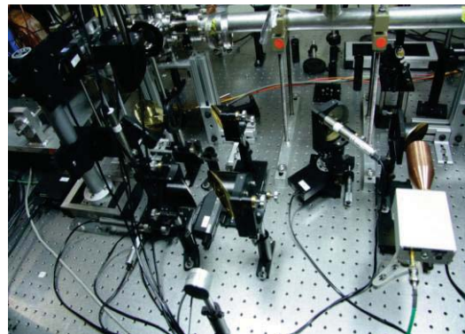
Figure 4: Layout of the THz diagnostic table and image of the current table setup.
