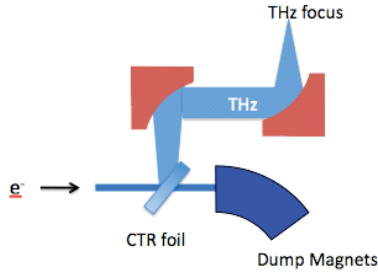
Figure 2: Schematic of thin-foil CTR THz generation, collection and focus.
