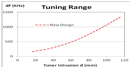
Figure 4: The cavity tuning curve.
