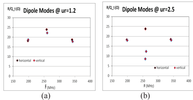
Figure 6: The dipole modes frequency spectrum at \mu_r=1.2 (a) and \mu_r=2.5 (b) with the tuner intrusion of 75 mm.
