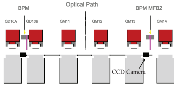
Figure 1: Layout of the Straightness Monitor installation in ATF2, showing the optical connections.
