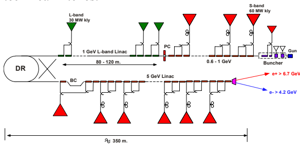
Figure 3: RF layout of the SuperB Injector.
