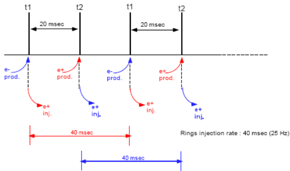
Figure 2: Timing process.
