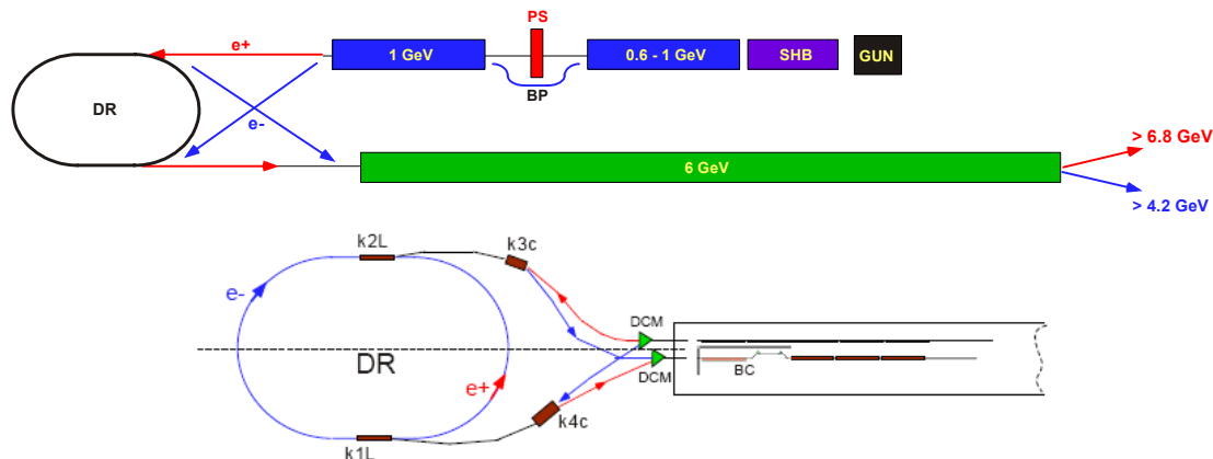
Figure 1: top) SuperB injector schematic layout; bottom) scheme of the transfer lines to/from the Damping Ring.
