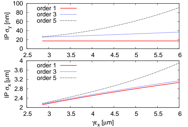
Figure 1: (top): Vertical beam size \sigma_y at the IP versus horizontal emittance for three different orders: first, third and fifth. Clearly the fifth order amplifies dramatically the beam size. (bottom): Horizontal beam size \sigma_x at the IP versus horizontal emittance
