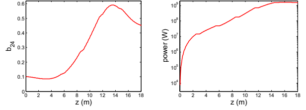
Figure 4: (a) Bunching factor vs radiator distance for the 10 nm radiation; (b) Peak power vs radiator distance for the 10 nm radiation.
