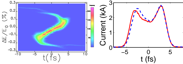
Figure 1: (Left) Longitudinal phase space for the under-compressed LCLS beam; (Right) True temporal profile (red) and predicted temporal profile (blue) from the longitudinal-to-transverse mapping technique (from Ref. [9]).
