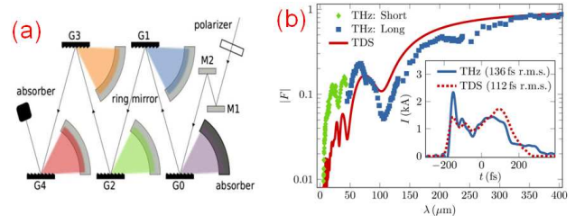
Figure 4: (a) Layout of the single-shot spectrometer; (b) Measured beam form factor from the spectrometer and that derived from measurement with a TCAV; the inset shows the beam temporal profile reconstructed from the spectrum and that from a TCAV (from [36]).
