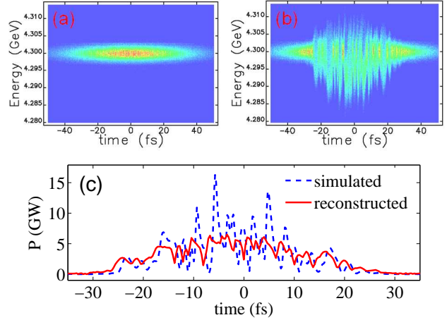
Figure 2: Beam longitudinal phase space with FEL off (a) and on (b); (c) X-ray power profile (provided by Y. Ding).
