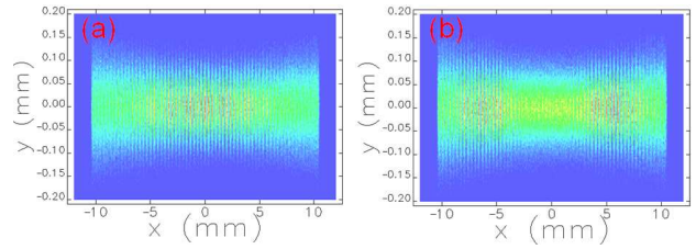
Figure 3: Simulated beam images for 5 keV energy modulation (a) and 12 keV energy modulation (b). Horizontal axis represents time.
