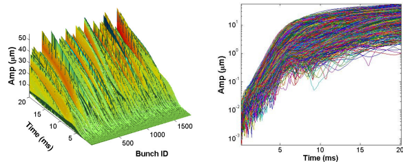
Figure 5. Simulated vertical beam ion instability in DRFS configuration. The vertical instability growth time is 0.91 ms .
