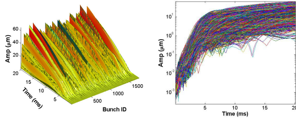
Figure 4. Simulated vertical beam ion instability in KCS configuration. The vertical oscillation amplitude in the left plot is in linear scale, while it is in logarithmic scale in the right plot. The different lines in the plots are for different bunches. The vertical instability growth time is 0.61 ms .
