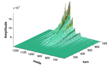
Figure 7. Unstable modes of the beam ion instability driven by ions in KCS configuration.
