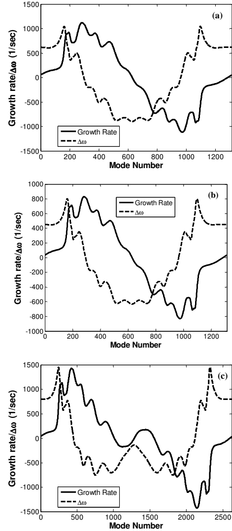
Figure 3. Calculated growth rate and frequency shift due to ions for different beams (a) KCS; (b) DRFS; (c) FP upgrade.
