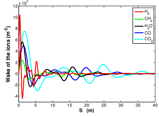
Figure 2. Wake field due to the ions along the whole ring with KCS beam. The total vacuum pressure is 0.5 nTorr with partial gas pressures shown in Table 1.
