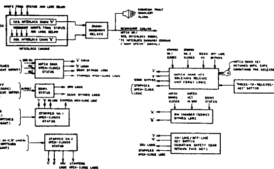
HUTCH CONTROL SYSTEM FUNCTIONAL LOGIC AND STATUS BLOCKS
