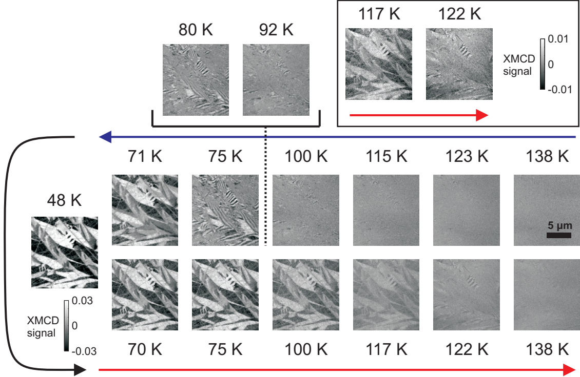
FIG. 2. (color online) PEEM data: XMCD images taken while cooling and warming the sample. Inset: The two images on either side of T_C , warming, with enhanced contrast to highlight the changes in the domain pattern across T_C . 48 K was the lowest temperature that we could achieve.
