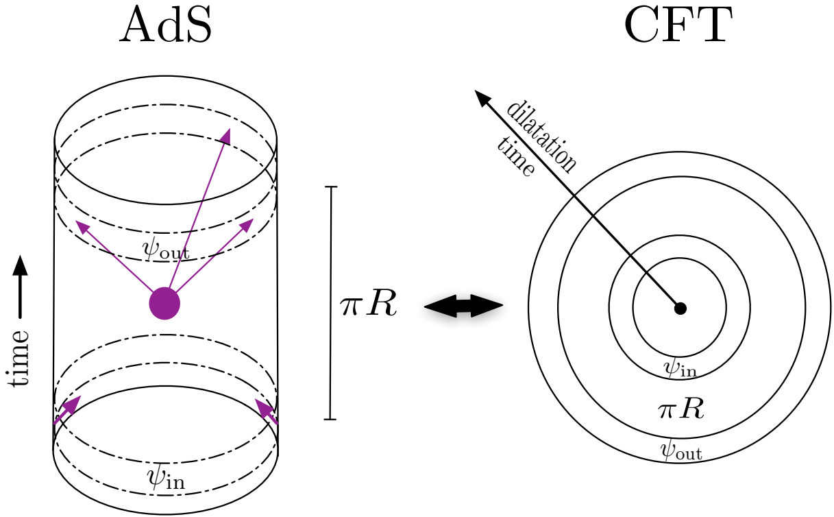
Figure 1: This figure shows how the \text{AdS}_{d+1} cylinder in global coordinates corresponds to the \text{CFT}_d in radial quantization. The time translation operator in the bulk of AdS is the dilatation operator in the CFT, so energies in AdS correspond to dimensions in the CFT. A scattering process in the bulk can be set up by acting with smeared CFT operators at an initial and final time that are separated by \pi R . In the large N limit, a product of n single-trace CFT operators creates an n -particle scattering state in the bulk.
