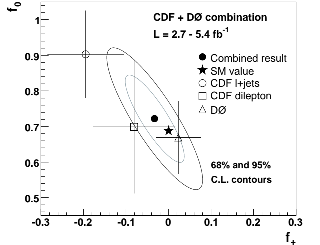
FIG. 1: Contours of constant \chi^2 for the combination of the 2D helicity measurements. The ellipses indicate the 68% and 95% C.L. contours, the dot shows the best-fit value, and the star marks the expectation from the SM. The input measurements to the combination are represented by the open circle, square, and triangle, with error bars indicating the 1\sigma uncertainties on f_0 and f_+ . Each of the input measurements uses a central value of m_t = 172.5 \text{ GeV}/c^2 .
