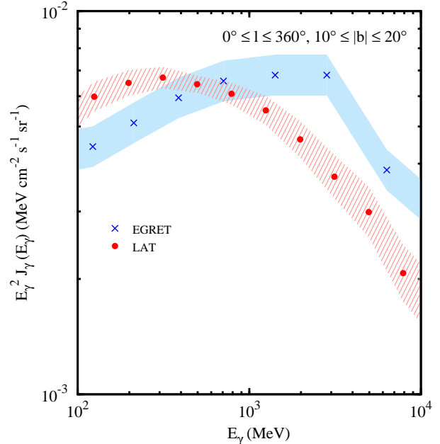
FIG. 1: Diffuse emission intensity averaged over all Galactic longitudes for latitude range 10^\circ \leq |b| \leq 20^\circ . Data points: LAT, red dots; EGRET, blue crosses. Systematic uncertainties: LAT, red; EGRET, blue.
