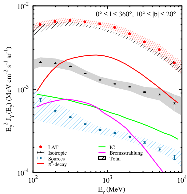
FIG. 2: LAT data with model, source, and UIB components for sky region in Fig. 1. Model (lines): \pi^0 -decay, red; bremsstrahlung, magenta; IC, green. Shaded/hatched regions: UIB, grey/solid; source, blue/hatched; total (model + UIB + source), black/hatched.
