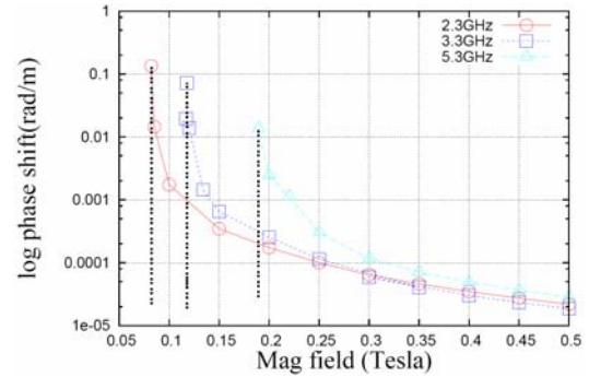
Figure 1. Calculated phase shift per unit length in a dipole region for a uniform cold electron plasma in a waveguide with 2 GHz cutoff frequency, the cloud density is assumed to be 1 \cdot 10^{12} \text{ e}^-/\text{m}^3 . The vertical lines correspond to an electron gyration frequency equal to the wave frequency.
