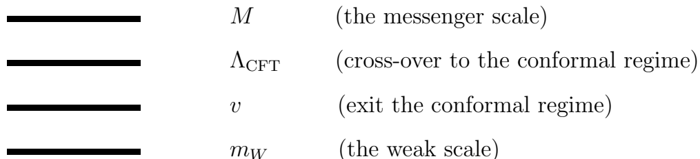
Figure 2: The relevant scales for our model.
