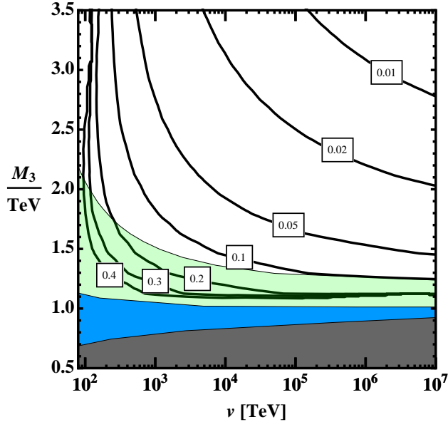
Figure 4: We plot contours of the “fine tuning” parameter \Delta^{-1} in the M_3 versus \nu plane. We make the same assumptions as in Fig. 3 with first/second generation squark masses at 5 TeV and \tan\beta = 2 . The solid grey region is excluded due to tachyonic third generation squarks, the solid blue region is excluded due to a lack of REWSB and the green translucent region is excluded due to the LEP bound on the A mass.
