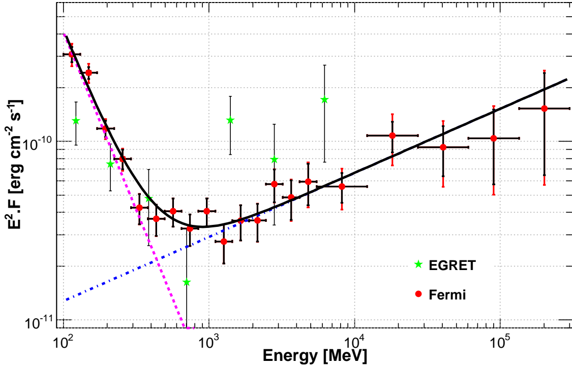
FIG. 5.— Spectral energy distribution of the Crab Nebula renormalized to the total phase interval. The fit of the synchrotron (purple dashed line) and IC (blue dashed-dotted line) are represented separately with two power-laws. The black curve is the best fit obtained with the sum of these two power-laws. The LAT spectral points are obtained using the model-independent maximum likelihood method described in Section 4.2. The statistical errors are shown in black, while the red lines take into account both the statistical and systematic errors. Horizontal bars delimit the energy intervals. EGRET data points (Kuiper et al. 2001) are shown for comparison (green stars).
