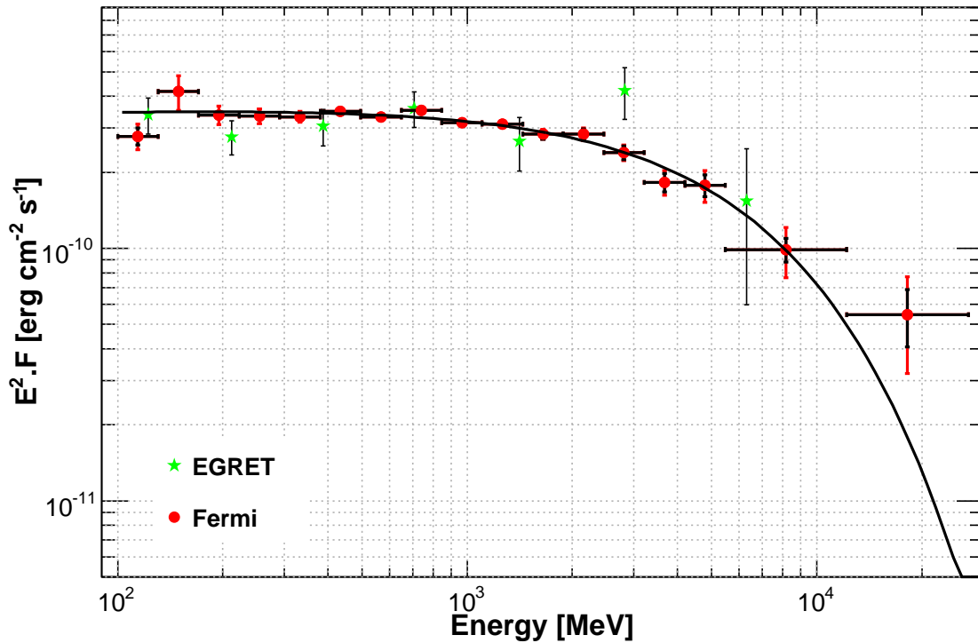
FIG. 6.— Spectral energy distribution of the Crab Pulsar averaged over the whole pulse period. The black curve represents the best fit model, obtained with a power-law with an exponential cut-off. The LAT spectral points (cf. Figure 5 for the description of the conventions) are obtained using the model-independent maximum likelihood method described in Section 4.2. EGRET data points (Kuiper et al. 2001) are shown for comparison (green stars).
