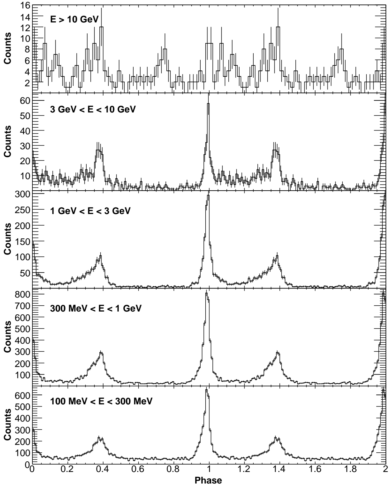
FIG. 3.— Fermi light curves for the Crab Pulsar in different energy bands within an energy-dependent circular region, as described in Section 4.1. The light curve profile is binned to 0.01 of pulsar phase, except above 10 GeV, which is binned to 0.02 in phase. Two cycles are shown.
