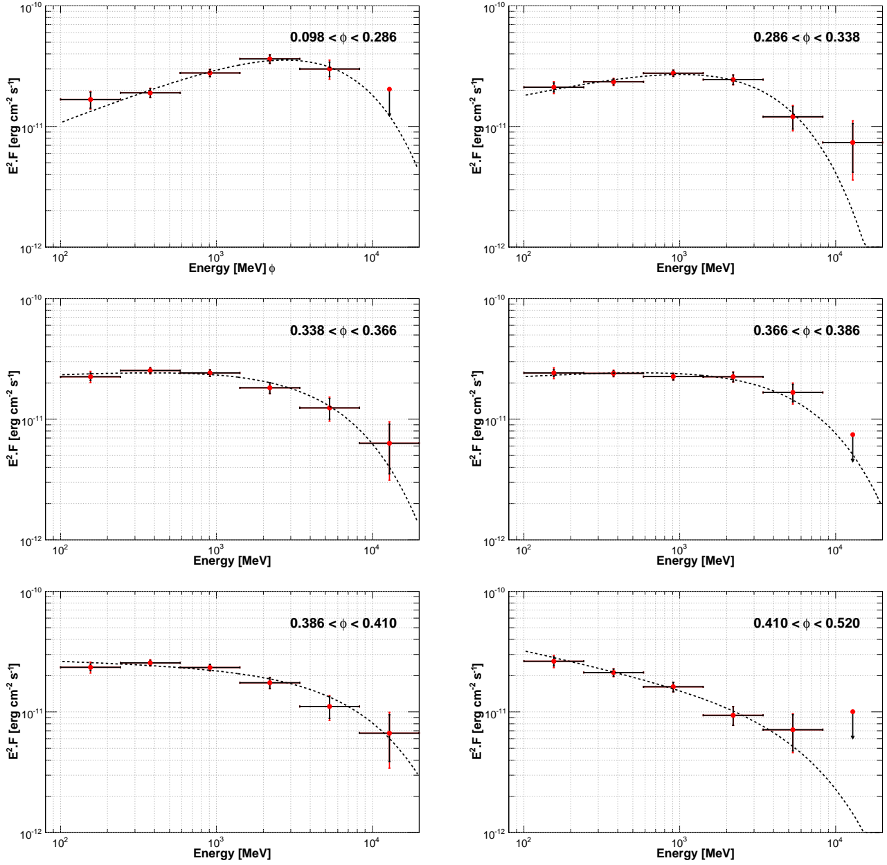
FIG. 7.— Phase-resolved spectral energy distributions of the Crab Pulsar. The labels indicate the phase intervals. Spectral results are presented in Table 2. The black dotted curve is the best fit power-law with an exponential cut-off. The LAT spectral points (cf. Figure 5 for the description of the conventions) are obtained using the model-independent maximum likelihood method described in Section 4.2. 90 % C.L. upper limits are computed when the statistical significance is lower than 3\sigma .
