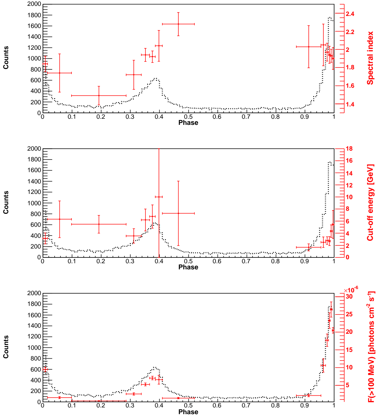
FIG. 8.— Variation of the spectral indices, cut-off energies and photon flux above 100 MeV (divided by the phase interval width) as the function of the pulse phase. A power-law with an exponential cut-off shape has been assumed for each phase interval (defined in Table 2). Vertical bars show the combined statistical and systematic errors. The horizontal bars delimit the phase interval containing \sim 1000 pulsed photons in the energy-dependent region defined in Section 4.1. The dotted histogram represents the Fermi -LAT lightcurve above 100 MeV, binned to 0.01 in phase.
