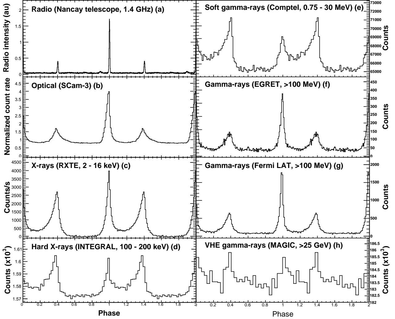
FIG. 2.— Light curves at different wavelengths. Two cycles are shown. References: (a) from the Nancay radio telescope; (b) Oosterbroek et al. (2008); (c) Rots et al. (2004); (d) Mineo et al. (2006); (e) Kuiper et al. (2001); (f) EGRET, Kuiper et al. (2001); (g) this paper; (h) Aliu et al. (2008).
