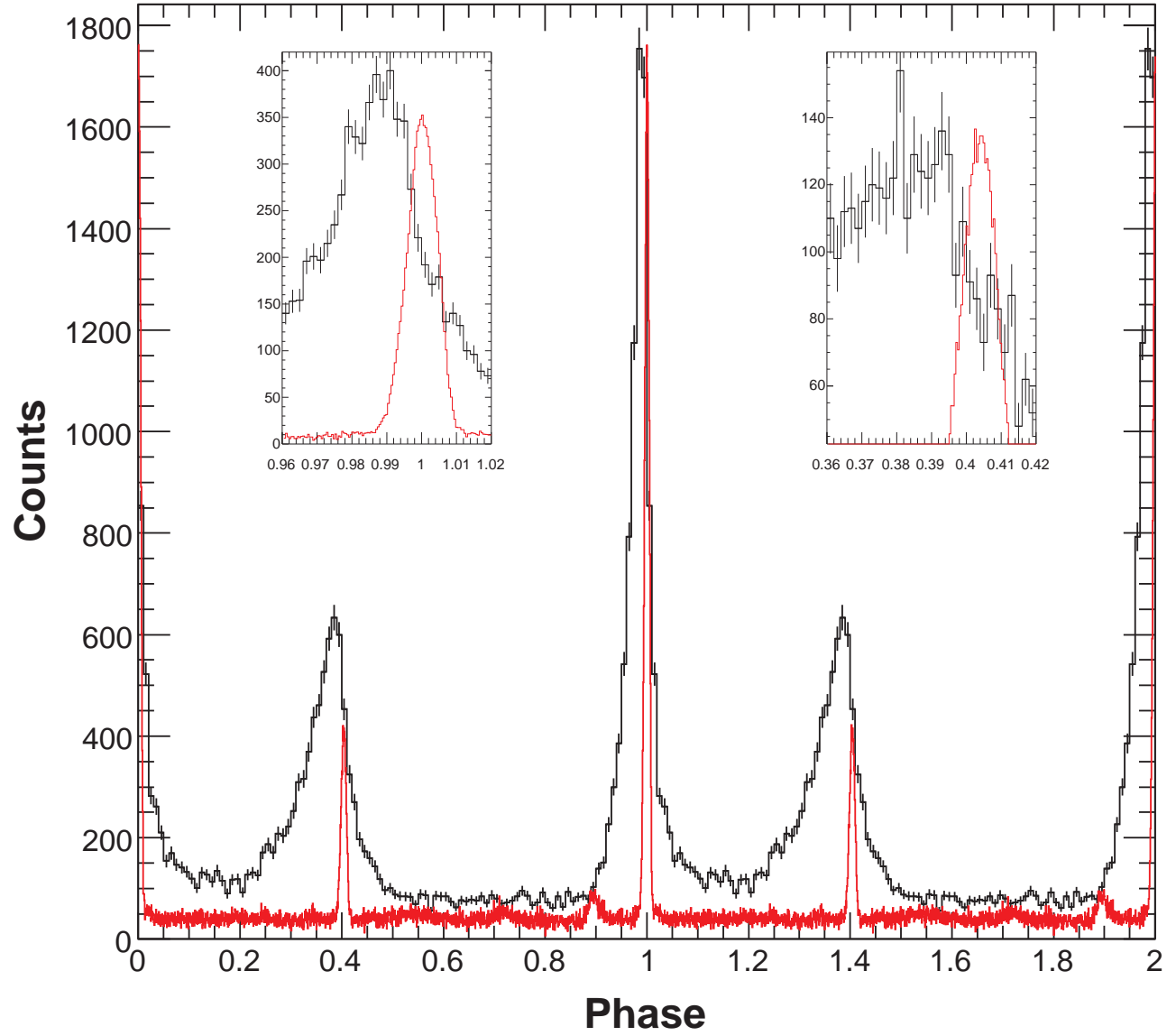
FIG. 1.— Light curve obtained with photons above 100 MeV within an energy-dependent circular region, as described in Section 4.1. The light curve profile is binned to 0.01 of pulsar phase. Insets show the pulse shapes near the peaks, binned to 0.002 in phase. The radio light curve (red line) is overlaid (arbitrary units). The main peak of the radio pulse seen at 1.4 GHz is at phase 0. Two cycles are shown.
