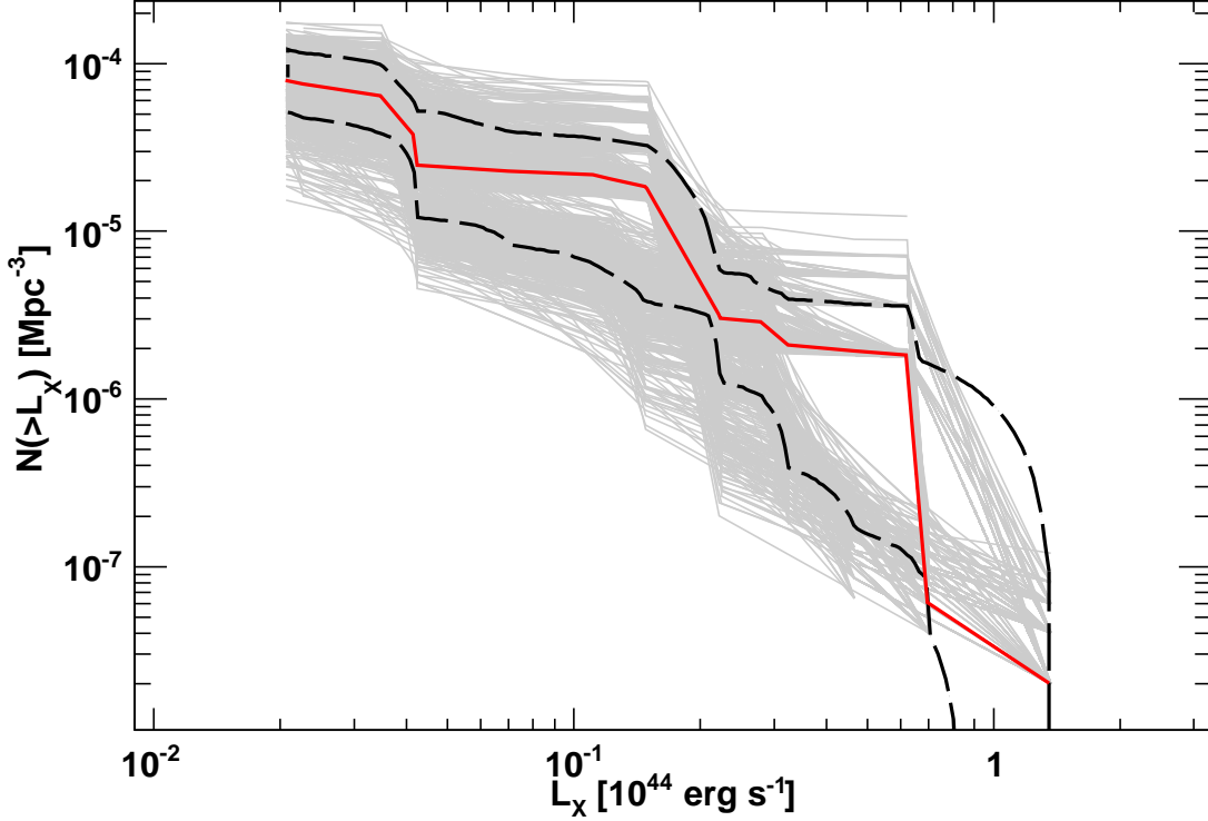
Fig. 7.— Cumulative space densities of Compton-thick AGN detected by BAT (thick red solid line) with 1\sigma confidence contours (dashed line) generated from the analysis of the bootstrapped samples (thin gray lines).
