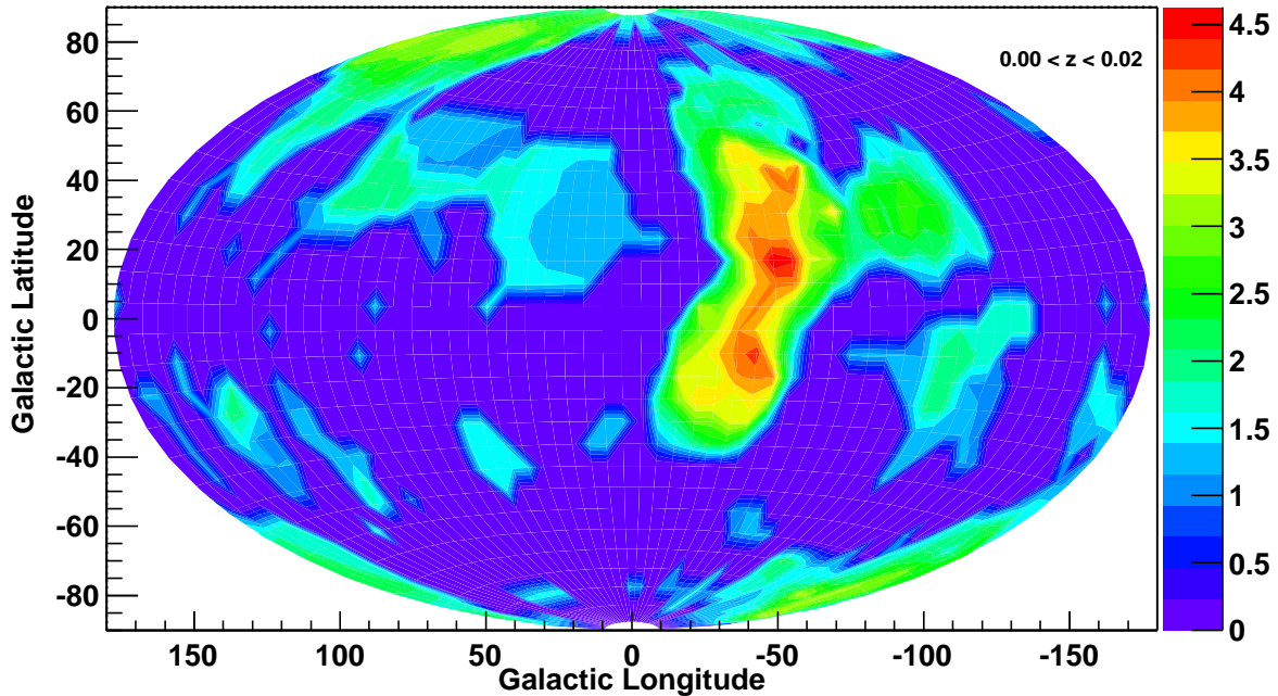
Fig. 9.— Significance of the density features of Fig. 8 expressed in number of \sigma .
