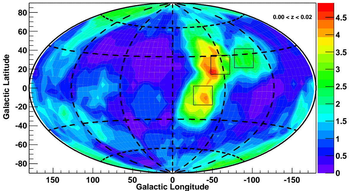
Fig. 8.— Fractional over-density of AGN with respect to the isotropic expectation within 85 Mpc. The color scale shows the ratio of BAT-detected AGN (within 20 degree cones) to the average number of AGN expected in the same area if sources were isotropically distributed. The map shows the regions where this ratio is the largest (red) and where it is the smallest (blue). The squares show the approximate position of the most prominent super-clusters (see text for details).
