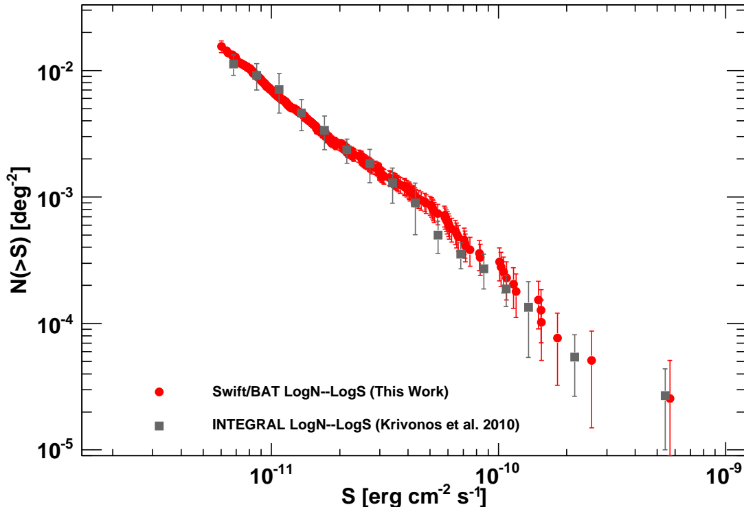
Fig. 4.— LogN-LogS of the BAT AGN in the 15–55 keV band (filled circles) compared to the one derived from INTEGRAL data by Krivonos et al. (2010) (squares)
