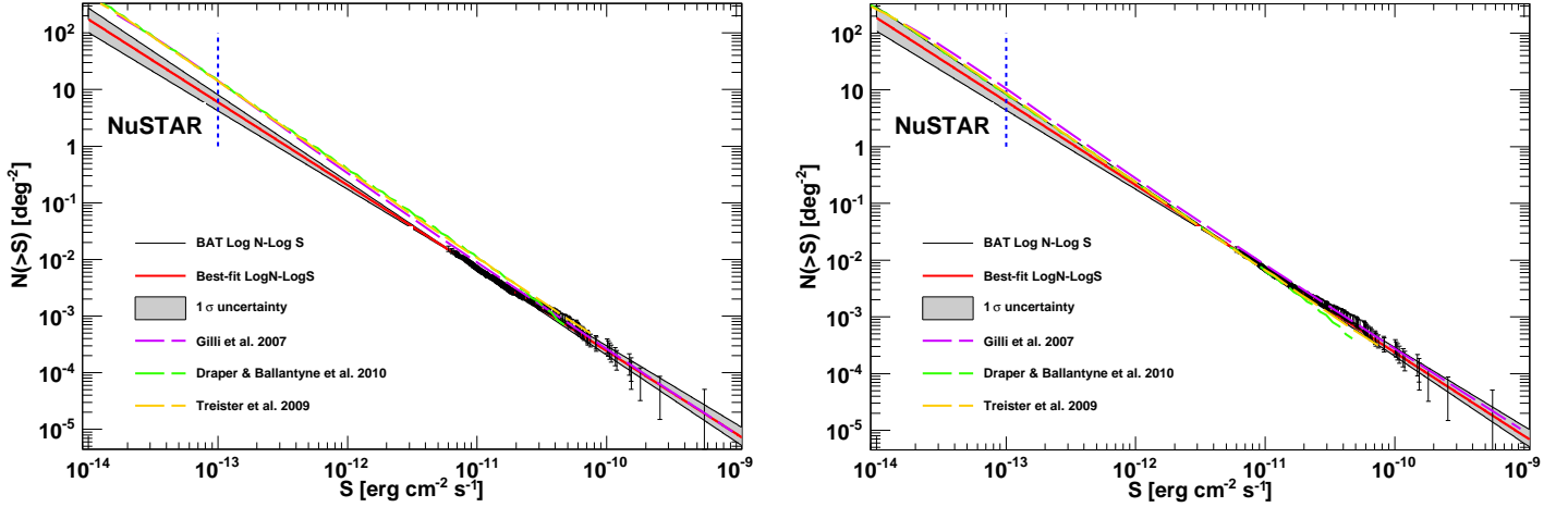
Fig. 11.— LogN-LogS of the BAT AGN (black data points) and best power-law fit extrapolated to the sensitivity that NuSTAR will achieve. The left panel shows the original prediction of synthesis models, while in the right panel the predictions have been renormalized to match the AGN densities measured by BAT. In both panels the vertical dashed line shows the sensitivity reached by NuSTAR in a short pointing (i.e. 5–10 ks).
