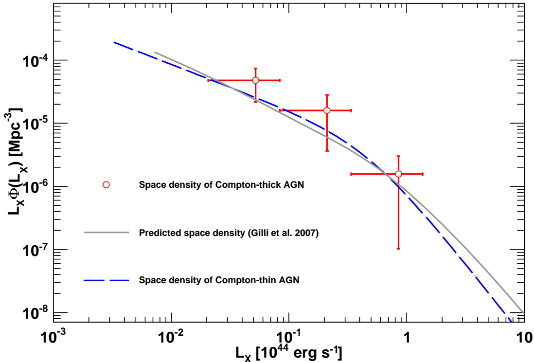
Fig. 6.— Space densities of Compton-thick AGN detected by BAT compared to model prediction from Gilli et al. (2007) and the space density of Compton-thin ( \text{Log}N_{\text{H}} < 24 ) AGN from § 3.2. Luminosities were de-absorbed following the method outlined in Burlon et al. (2011).
