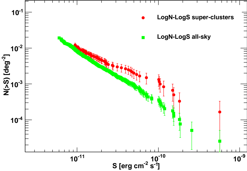
Fig. 10.— LogN–LogS (15–55 keV) of the AGN in the direction of the Hydra-Centaurus super-clusters and of the Great Attractor compared to the LogN–LogS of all AGN.
