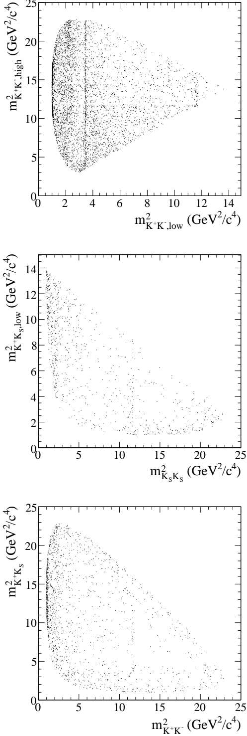
FIG. 1: Dalitz plots for B^+ \rightarrow K^+K^-K^+ (top), B^+ \rightarrow K_S^0 K_S^0 K^+ (middle), and B^0 \rightarrow K^+K^-K_S^0 (bottom). Points correspond to candidates in data that pass the full event selection, with an additional requirement that the NN output be 7 or less, in order to enhance the signal.
