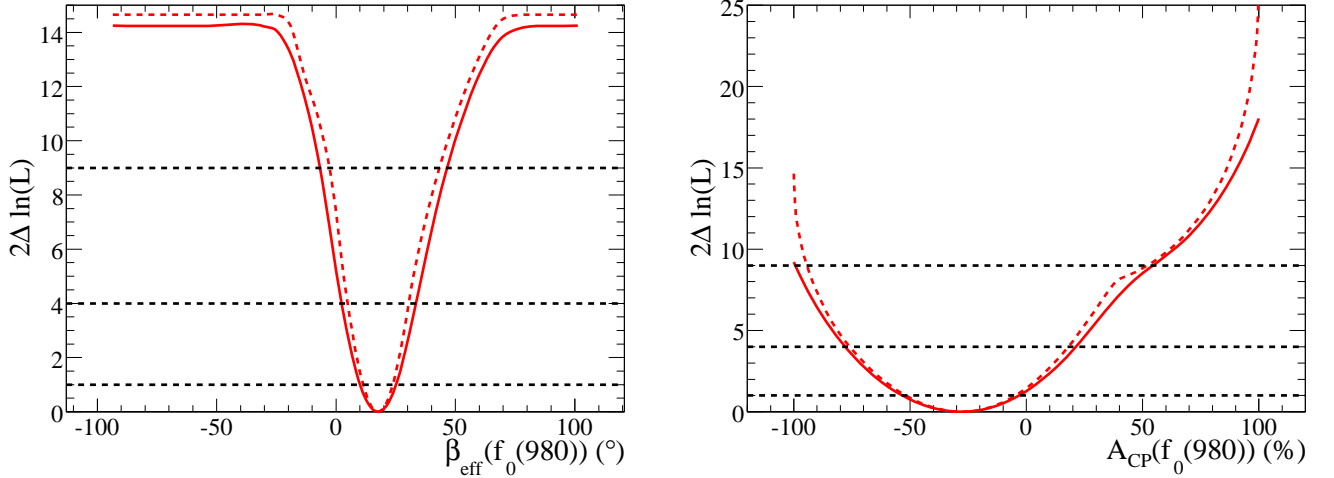
FIG. 20: Scan of 2\Delta \ln \mathcal{L} , with (solid line) and without (dashed line) systematic uncertainties, as a function of \beta_{\text{eff}} (left) and A_{CP} (right) for B^0 \rightarrow f_0(980)K_s^0 . The flat region of the \beta_{\text{eff}} scan is caused by the A_{CP}(f_0(980)) going to -100\% in this region, in which case \beta_{\text{eff}} becomes an irrelevant parameter.
