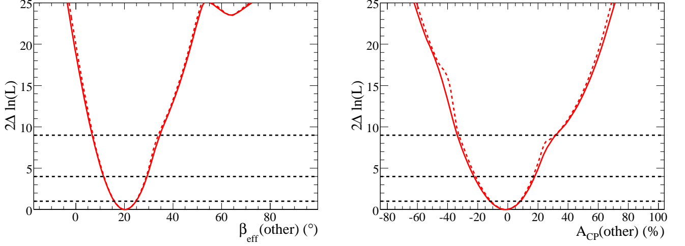
FIG. 21: Scan of 2\Delta \ln \mathcal{L} , with (solid line) and without (dashed line) systematic uncertainties, as a function of \beta_{\text{eff}} (left) and A_{\text{CP}} (right) for B^0 \rightarrow K^+ K^- K_S^0 , excluding the \phi(1020) , f_0(980) , and \chi_{c0} .
