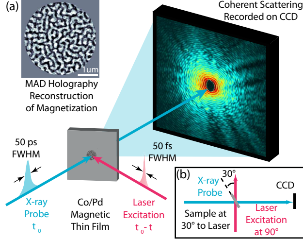
FIG. 1. Schematic of optical pump x-ray probe experimental setup. a) Sample magnetization reconstructed using MAD Holography[13]. b) Overhead schematic of experimental geometry.
