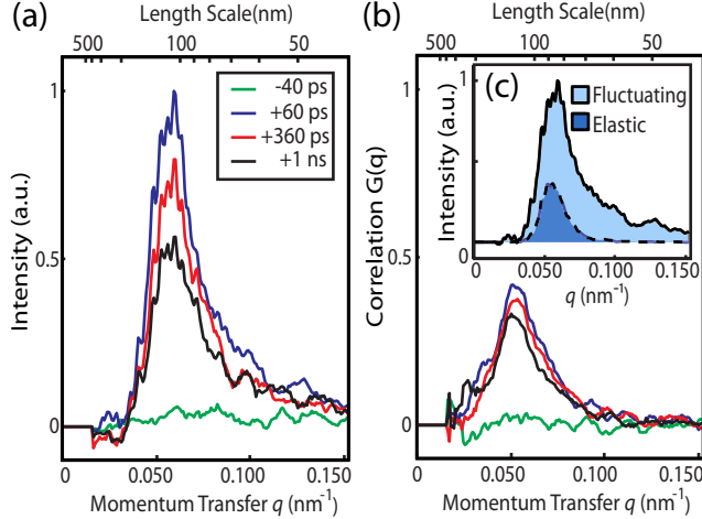
FIG. 3. a) Radial integration of the normalized difference for different time delays. b) Corresponding q dependent correlation to the normalized difference at 0 ps. c) Shown for the +60 ps signal, by multiplying panels a and b, the elastic and fluctuating portions of the magnetization changes can be identified.
