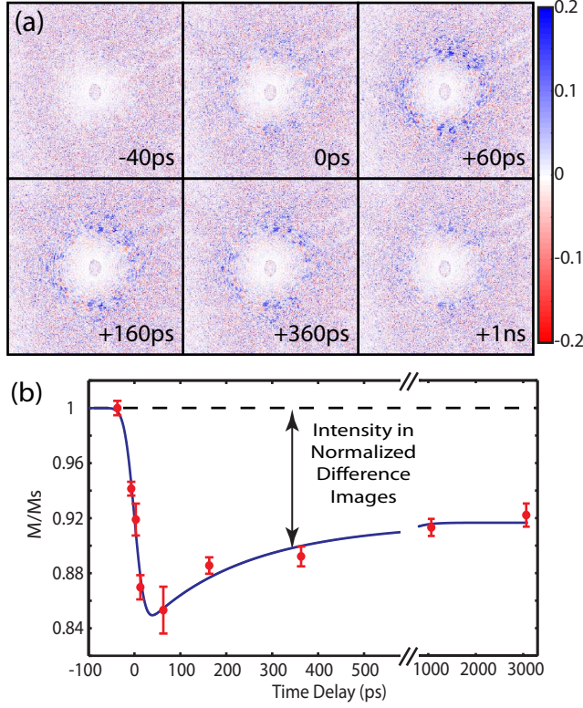
FIG. 2. a) Normalized change in magnetic scattering at various time delays. The q range extends out to 0.125 \text{ nm}^{-1} . The stable speckle configuration indicates that the underlying domain structure is maintained. b) Demagnetization curve from \Delta I_{\text{norm}} , which is proportional to deviation from M/M_s = 1 . The line is a fit to the data with Koopman’s micro three temperature model [20], which indicates a demagnetization of 20-25%. The plotted curve is significantly broadened by convolution with a 50 ps FWHM Gaussian corresponding to the width of the x-ray probe.
