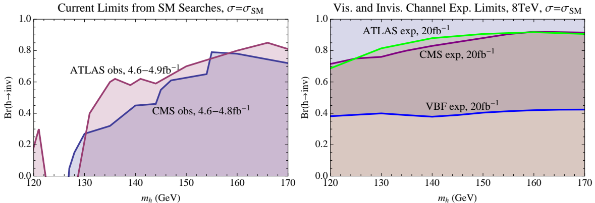
Figure 6: Left: Present observed lower bound on the invisible branching ratio assuming the IHH. Right: Expected lower limit from visible channels and upper limit from the WBF invisible channel with 20 \text{ fb}^{-1}/\text{channel} at 8 TeV.
