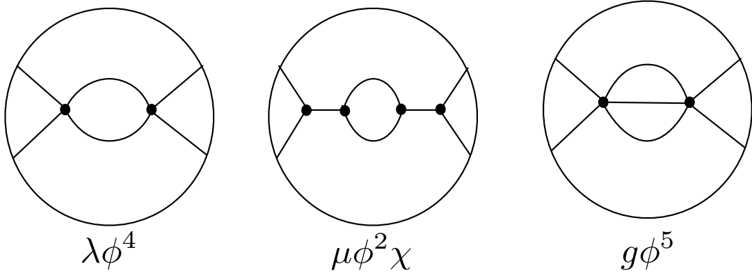
Figure 5: This figure shows the 1-loop and 2-loop diagrams that we have computed using the Mellin space version of the Källén-Lehmann representation. Further generalizations are straightforward.
