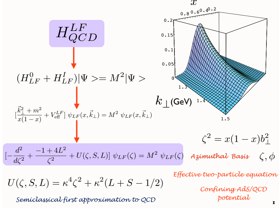
Fig. 2. – Reduction of the Light-Front Hamiltonian to an effective LF Schrodinger Equation for mesons. The insert shows the AdS/QCD – light-front holography prediction for the pion’s valence LFWF \psi(x, \vec{k}_\perp) . From ref. [30].
