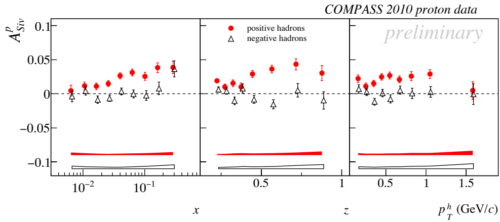
Fig. 4. – Preliminary measurements of the Siverts single-spin asymmetry by COMPASS in deep inelastic muon-proton scattering.
