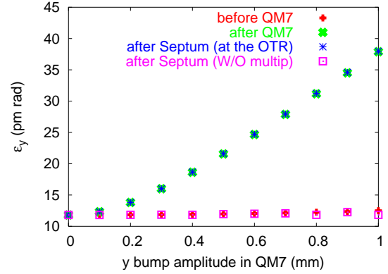
Figure 1: Emittance vs vertical bump amplitude in QM7 at different locations of the EXT line, from tracking simulations with and without the multipole coefficients in Table 1.
