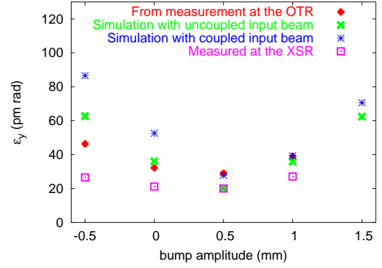
Figure 3: Projected vertical emittances at the OTR and XSR computed from \beta_y -functions and measured beam sizes, and emittances obtained from tracking simulations.
