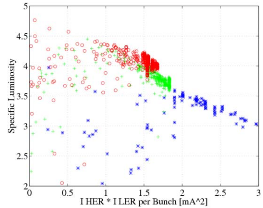
Figure 11 : Specific luminosity versus the product of the bunch currents. The specific initially rises because of dynamic beta effects and then falls due to beam-beam interaction from both primary and parasitic collisions. The parasitic beam-beam effect was only a few percent. The blue points are By-4 pattern scaled to the By-2 pattern.
