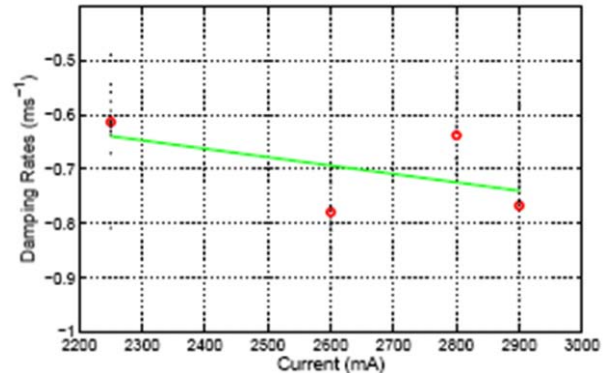
Figure 7 : LER longitudinal feedback damping rates with total positron current.
