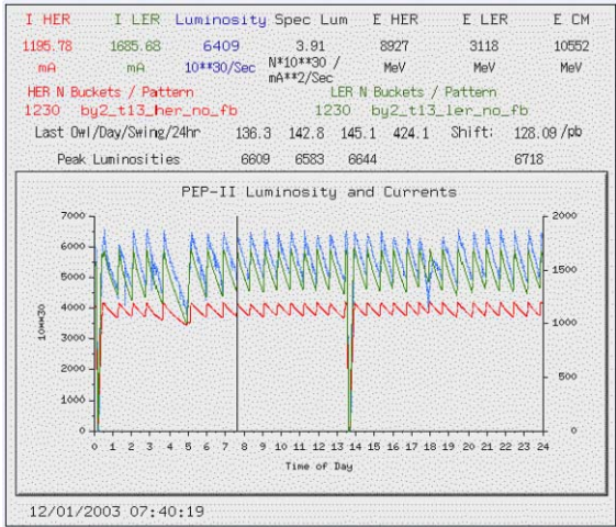
Figure 12 : Luminosity and beam currents for 24 hours showing the fill-coast mode of PEP-II in early years.
