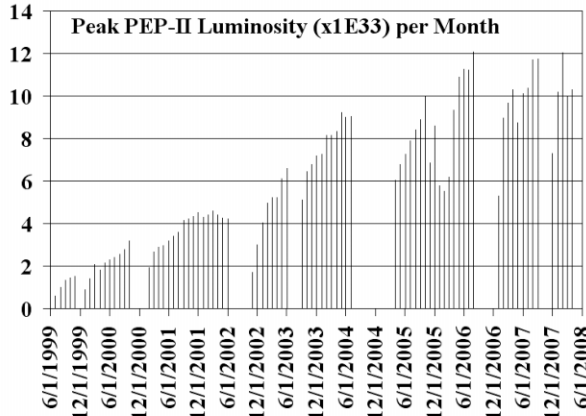
Figure 16 : Peak luminosity in a given month from 1999 to 2008. A peak luminosity of 1.21 \times 10^{34}/\text{cm}^2/\text{s} was achieved.
