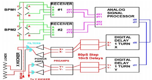
Figure 6 : Bunch-by-bunch transverse feedback system.
