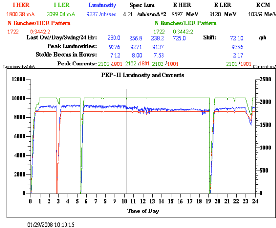
Figure 13 : Continuous injection of both PEP-II beams.
