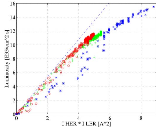
Figure 10 : Luminosity versus the product of the bunch currents. The red and green curves show luminosity in the By-2 pattern (4 nsec) bunch spacing during routine operation achieving a luminosity of 1.2 \times 10^{34} . The blue curve shows the By-4 bunch pattern (8 nsec) scaled to a By-2 bunch pattern, indicating an increased luminosity may have been possible in PEP-II with the By-2 pattern.
