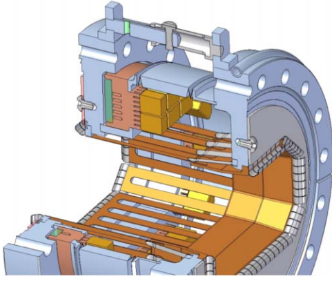
Figure 8 : Ultimate design of the PEP-II high power expansion bellows module with sliding fingers, compression (hold down) fingers, beam RF seals at the ends, and water cooled HOM absorbing tiles.
