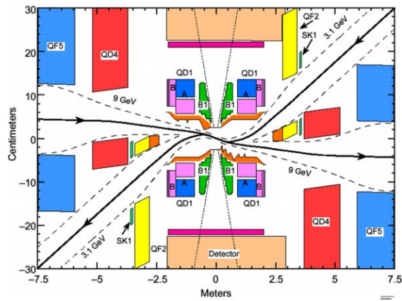
Figure 2 : PEP-II Interaction Region (IR) with head-on collisions. There are four permanent magnets within the BaBar 1.5 T solenoidal field covering \pm 2.5 m.
