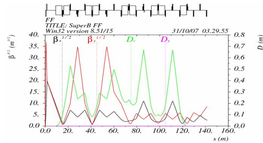
Figure 3: Optical functions in half IR, IP is at s=0 , crab sextupole at s=140 .
