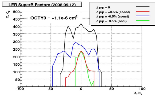
Figure 4: LER dynamic aperture (preliminary).
