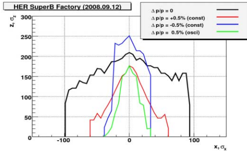
Figure 5: HER dynamic aperture (preliminary).
