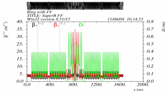
Figure 1: LER optical functions.
