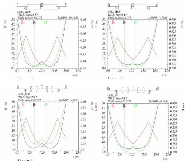
Figure 2: HER (top) and LER (bottom) arc cells:
