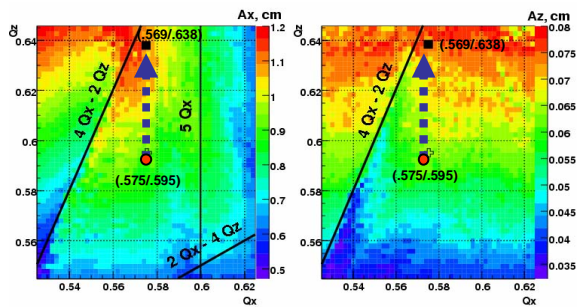
Figure 6: Example of HER DA vs tune scan.
