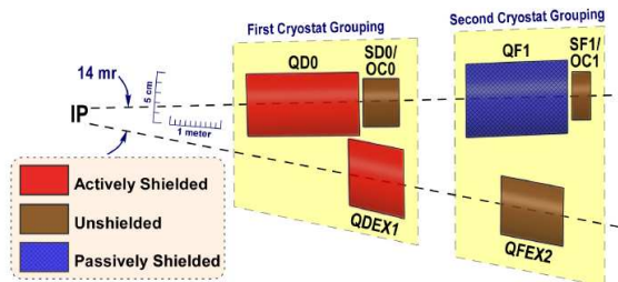
Figure 1: ILC IR layout [1].
