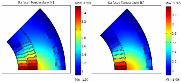
Figure 5: The calculated temperature profile in the 4-layer and 2-layer IR quadrupole magnets.
